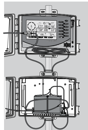
Wireless Vantage Pro2 console mounted in Extra Solar Power Kit (top) with Heavy Duty Solar Power Kit (6612, bottom)
