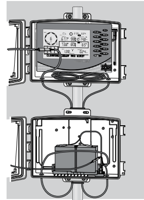
Cabled or wireless (shown) Vantage Pro2 console mounted in Universal Shelter (6618, top) with Heavy Duty Solar Power Kit (bottom)
