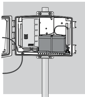
Cabled Weather Envoy with Heavy Duty Solar Power Kit
