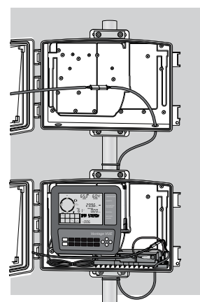
Vantage Vue Console mounted in Solar Power Kit (6614, bottom) with Extra Solar Panel Kit (top)
