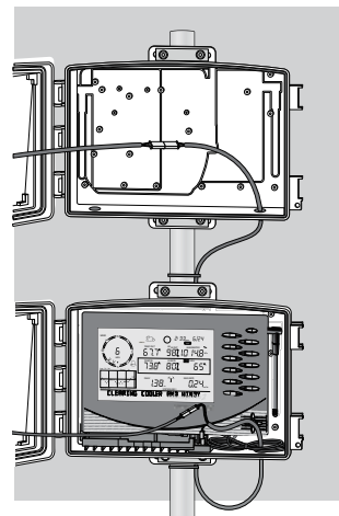
Wireless Vantage Pro2 console in Solar Power Kit (bottom) and Extra Solar Panel Kit (top)
