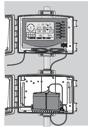
Cabled Vantage Pro2 console in Universal Shelter (6618, top) with Heavy Duty Solar Power Kit (bottom)
